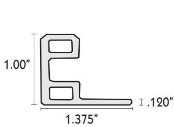
DECK STARTER
