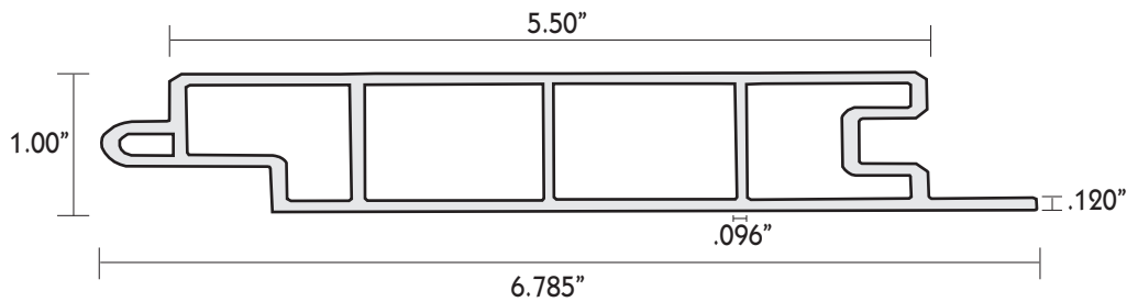
DECK BOARD
