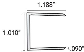
C-CHANNEL
